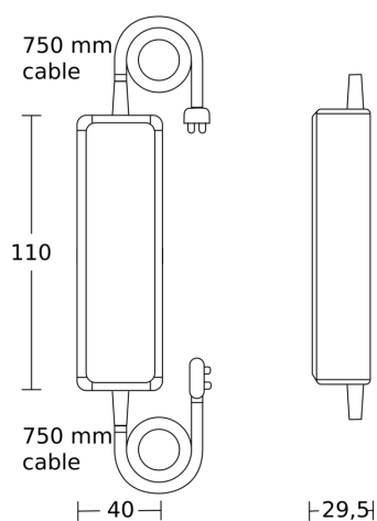
Dimension Drawing 2
